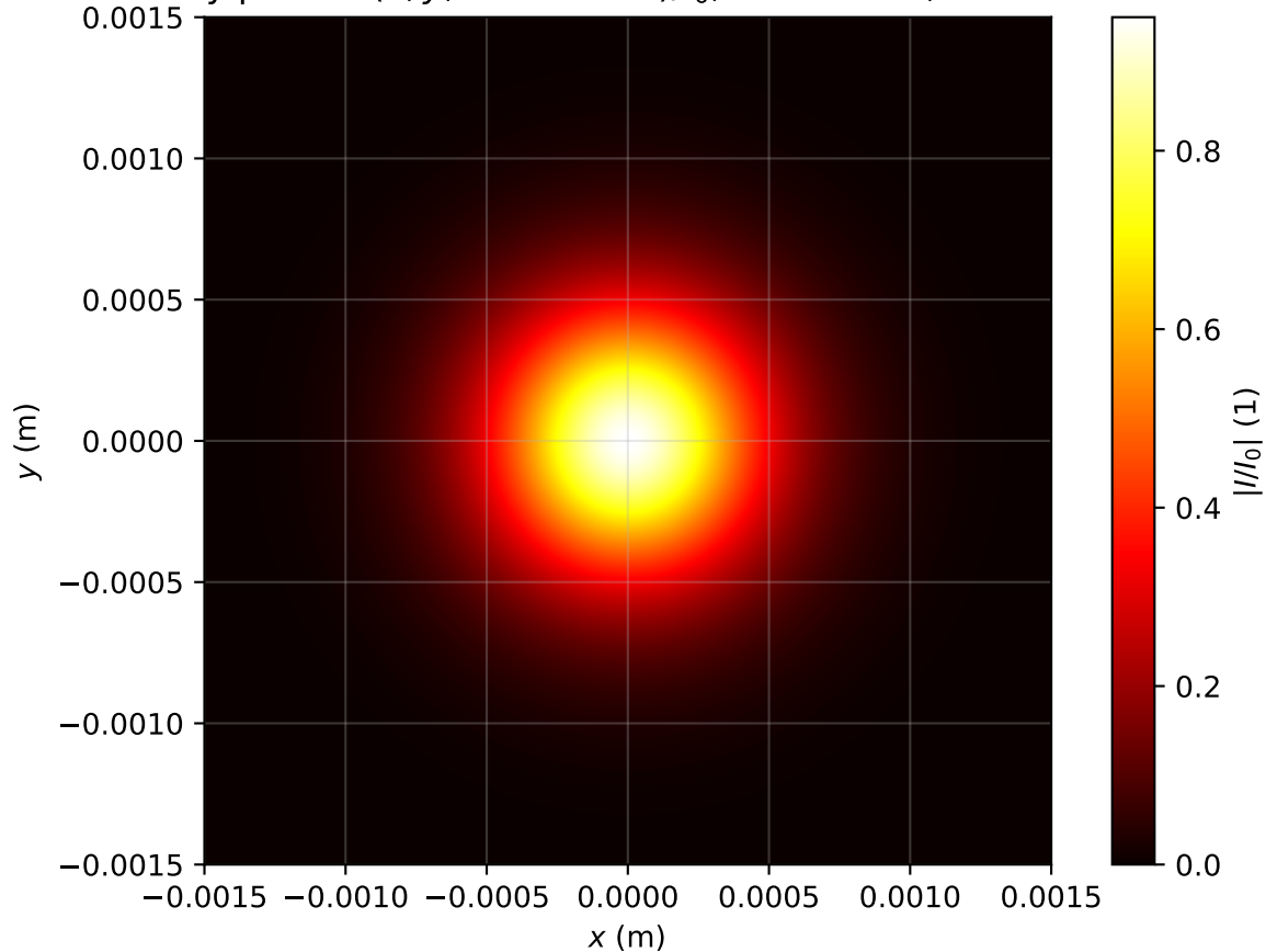
Intensity profile I(x, y, z = 1.194m)/I_0 , \text{Pin}=0.4\text{Pcr} , artificial time
